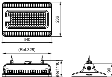
High-bay/ low-bay LED
