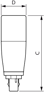
PLED 220-240V 11-26W 1400lm 6500K G24D
