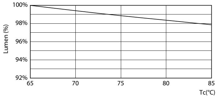
LEDtube PLC 11W 15K 3 LumenVsTc
