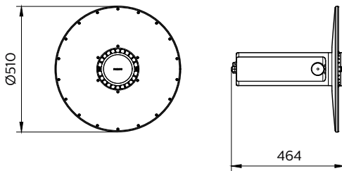
BY718P GreenPerform Highbay Elite
