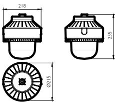
BY200P LED44 L-B/NW PSU
