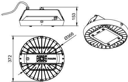
BY689P LED110/CW PSU NB G2 XT
