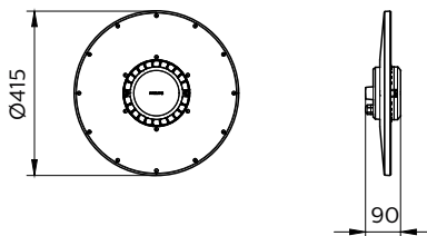
BY718P LED150/NW PSU WB NCH
