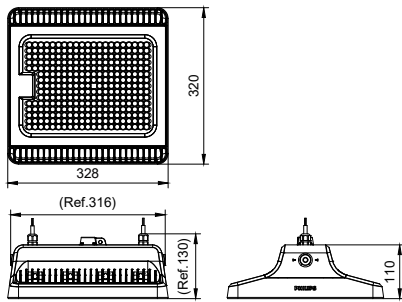
BY570P LED250/CW PSU HRO GC
