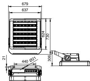
BVP621 LED1110/757 900W SP PSD GC O
