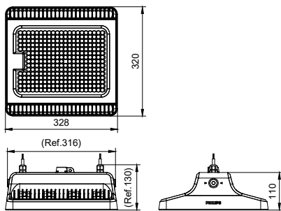
BY570P LED250/CW PSD NB GM
