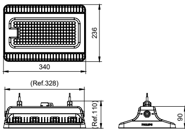
BY570P LED150/840 PSU NB CAU
