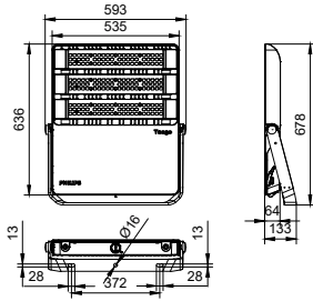
BVP384 LED614/NW 490W 220-240V AWB GC
