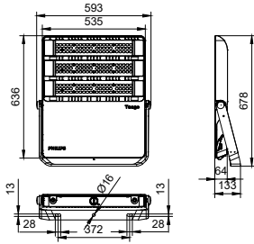
BVP384 LED614/NW 490W 220-240V NB GC
