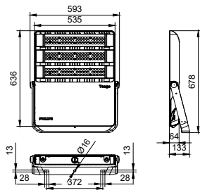
BVP384 LED614/CW 490W 220-240V S6 GC
