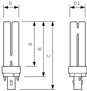
PL-C 10W/865/2P
