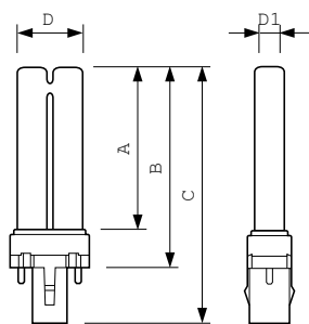
MASTER PL-S 11W/840/2P 1CT/10
