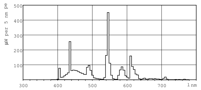
LDPB_PLC2P_865-Spectral power distribution B/W
