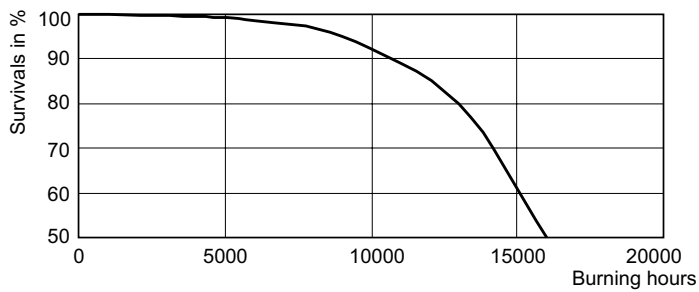
Life Expectancy Diagram - MASTERC CDM-TP 150W/942 PGX12-2 1CT/12
