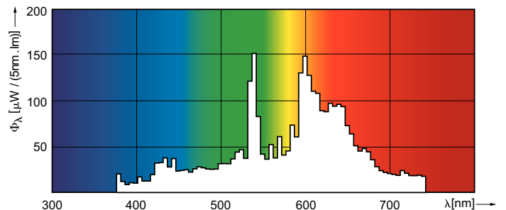
Spectral Power Distribution Colour - MASTERC CDM-T Elite 35W/930 G12 1CT/12
