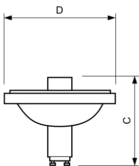
MASTERColour CDM-R111 Elite CDM-R111 Elite 70W/930 GX8.5 40D
