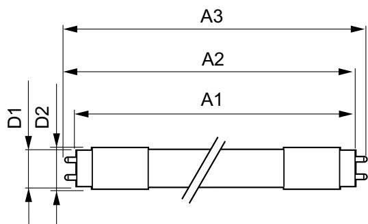
MASTER LEDtube 1200mm HO 14W830 T8
