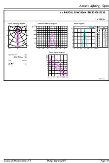
LEDspot MAS 20W E27 PAR30L 830 15D ND
