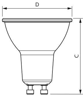
MC LEDspot IA 4.7-50W GU10 927 36D CN
