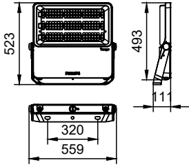
Floodlight surface LED
