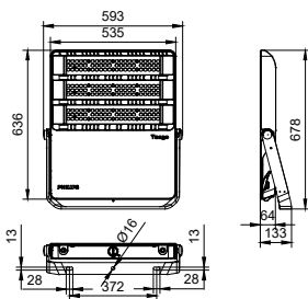
BVP384 LED733/757 580W 220-240V NB GM
