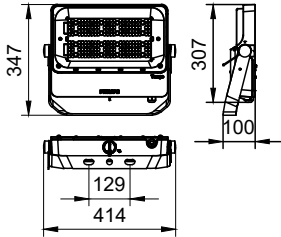
BVP432 LED274/NW 220~240V 200W SWB GC
