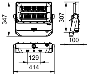
BVP432 LED272/CW 220~240V 200W SWB GC
