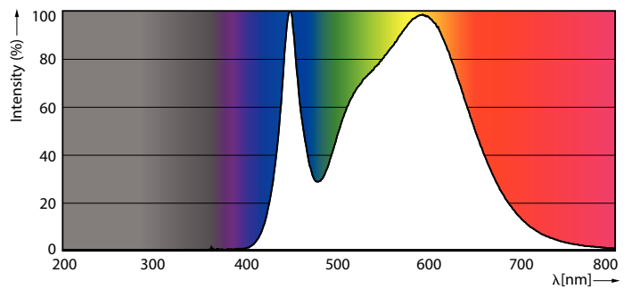
LEDTForce Core GC 50W Tshape E27 840-POC
