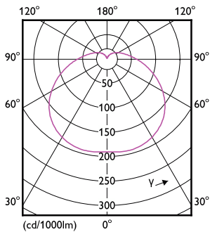
LEDTForce Core GC 50W Tshape E27-LDD
