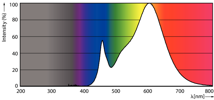
LEDtube PLC 11W G24D 1250lm 830
