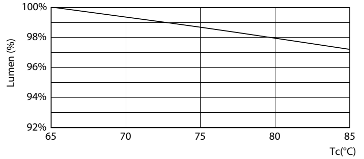
LEDtube PLC 11W 15K 1 LumenVsTc
